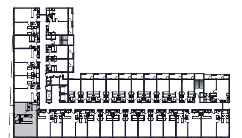
1ST-2ND FLOOR LEVEL
