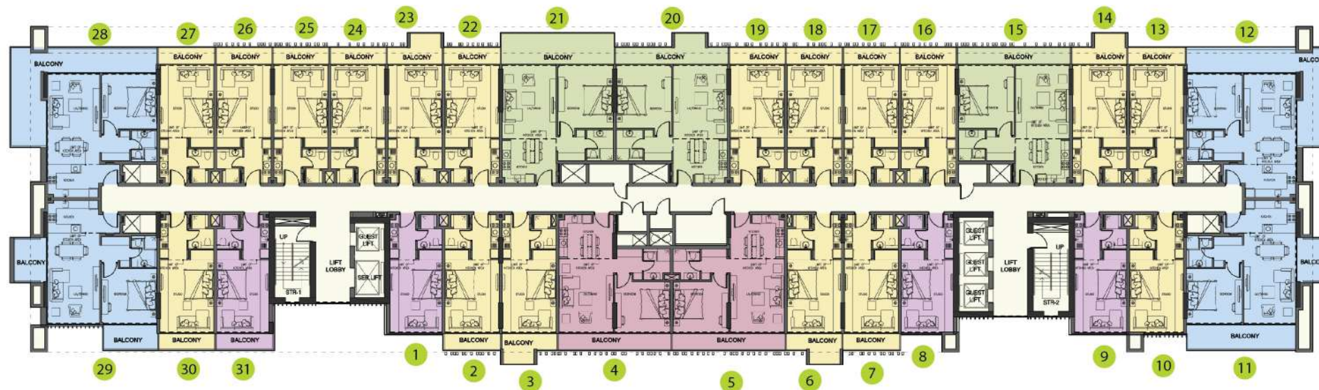
8th Floor Plan
