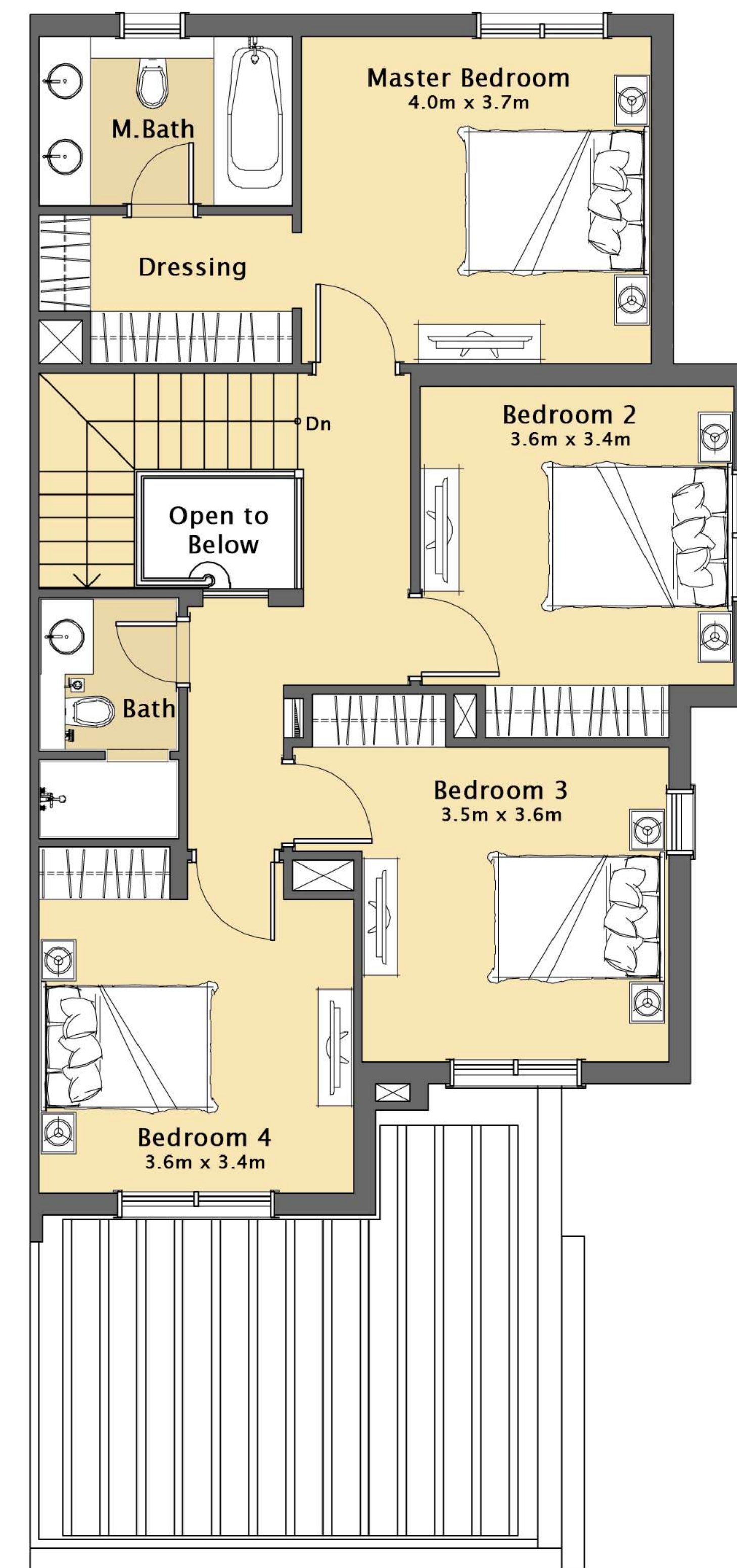
FIRST FLOOR
