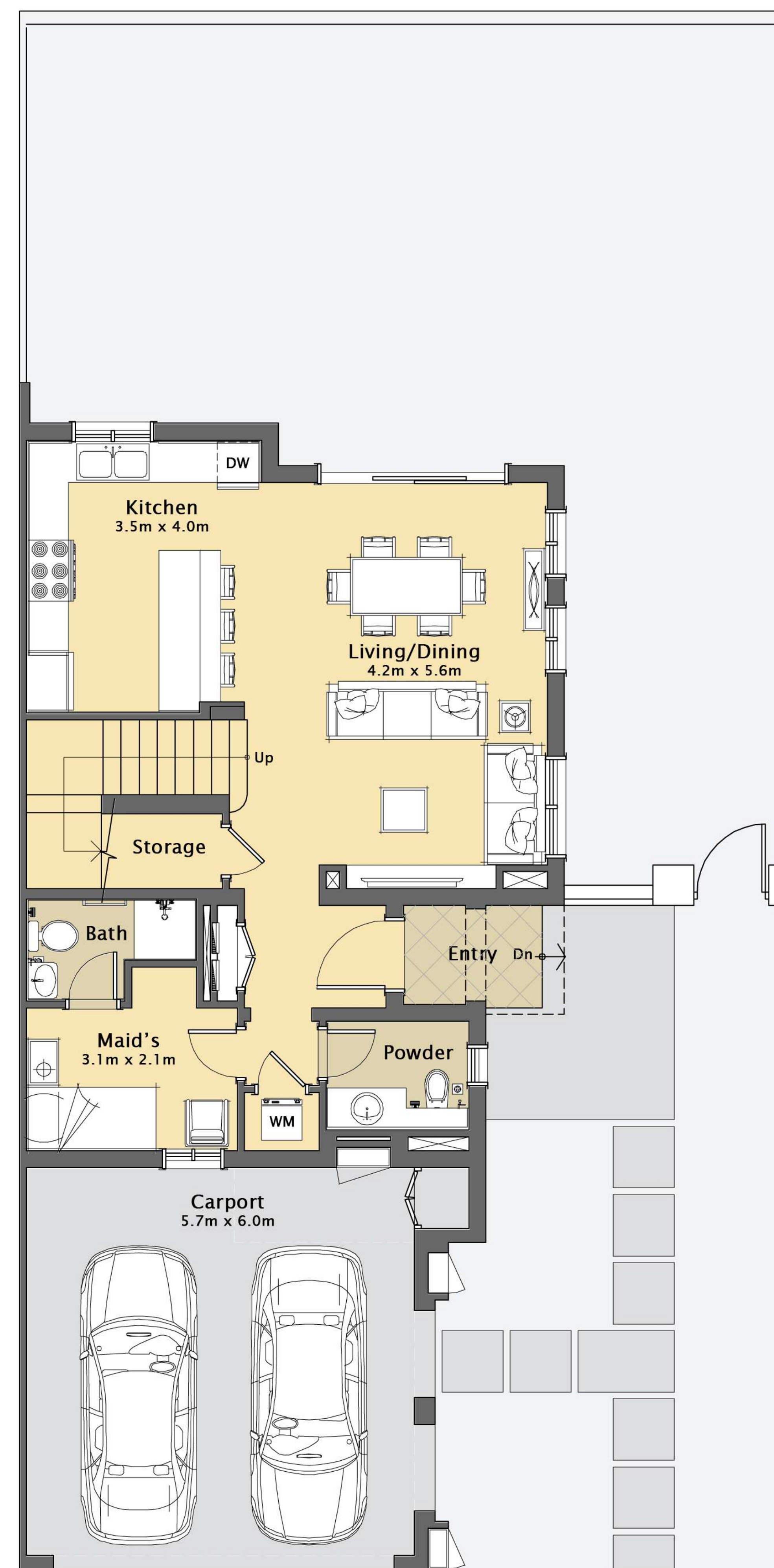
GROUND FLOOR
