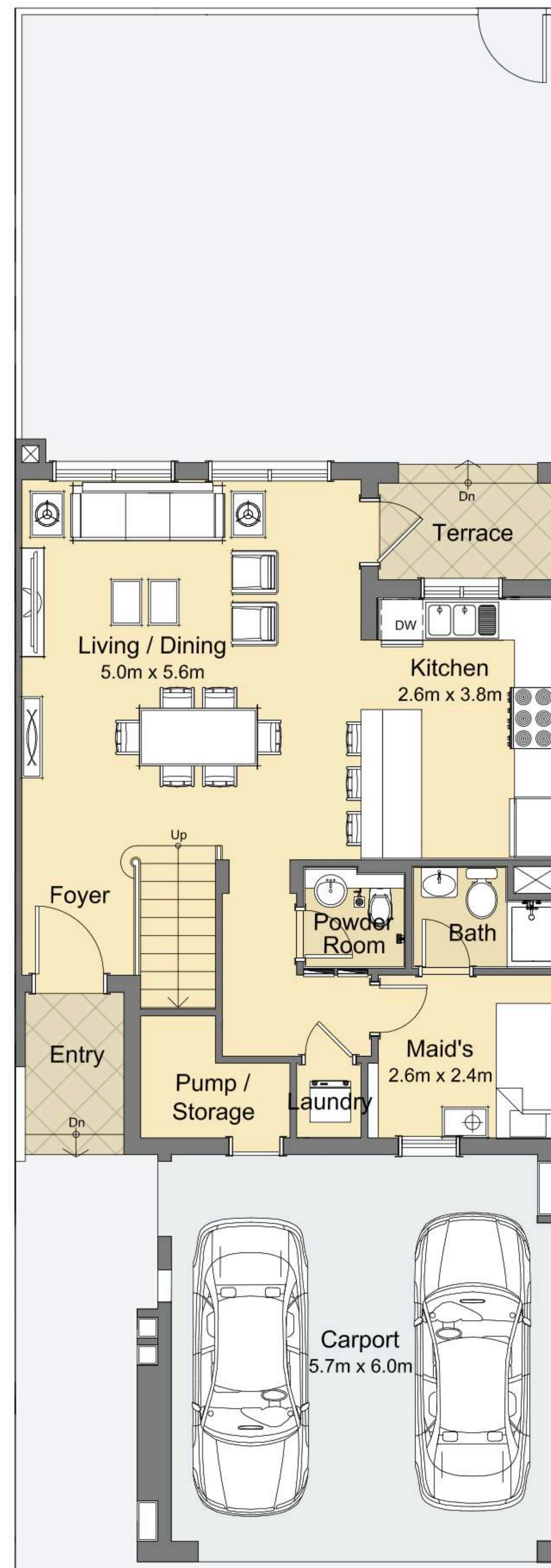
GROUND FLOOR
