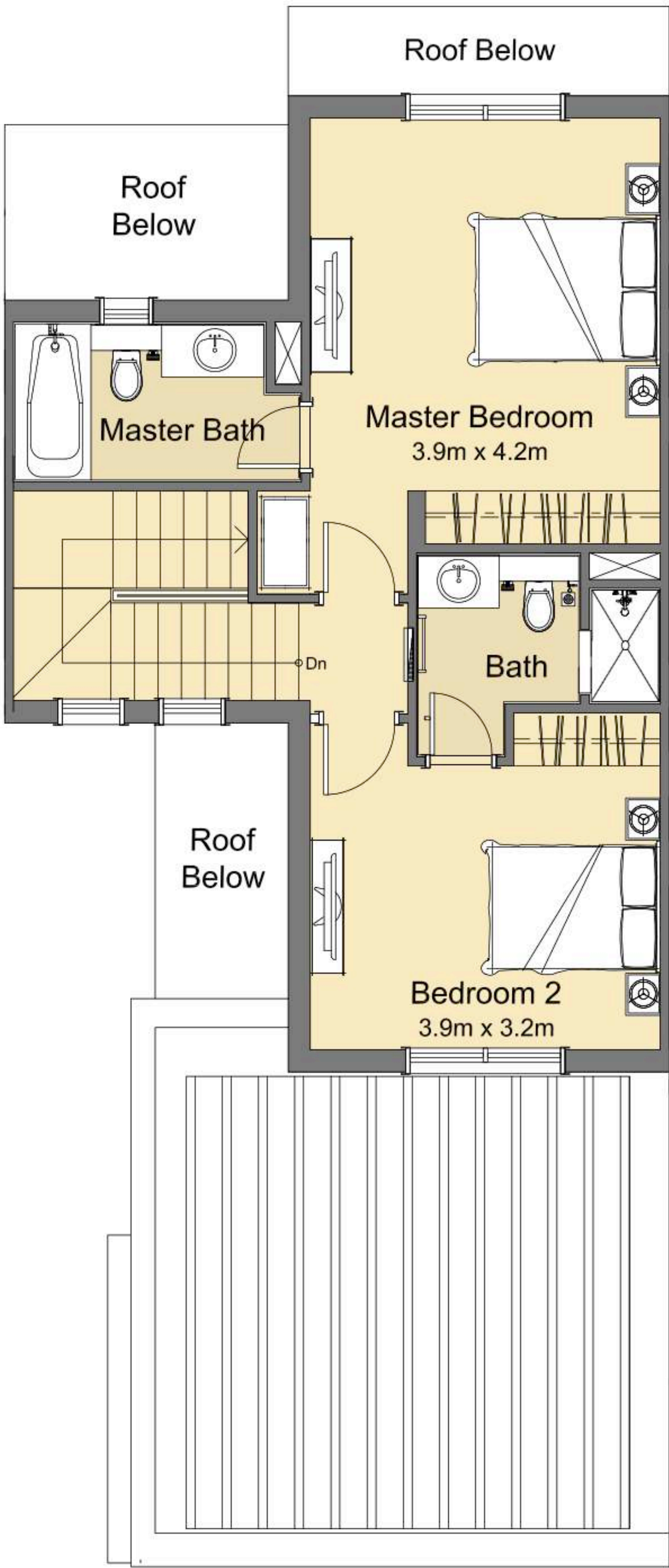
FIRST FLOOR
