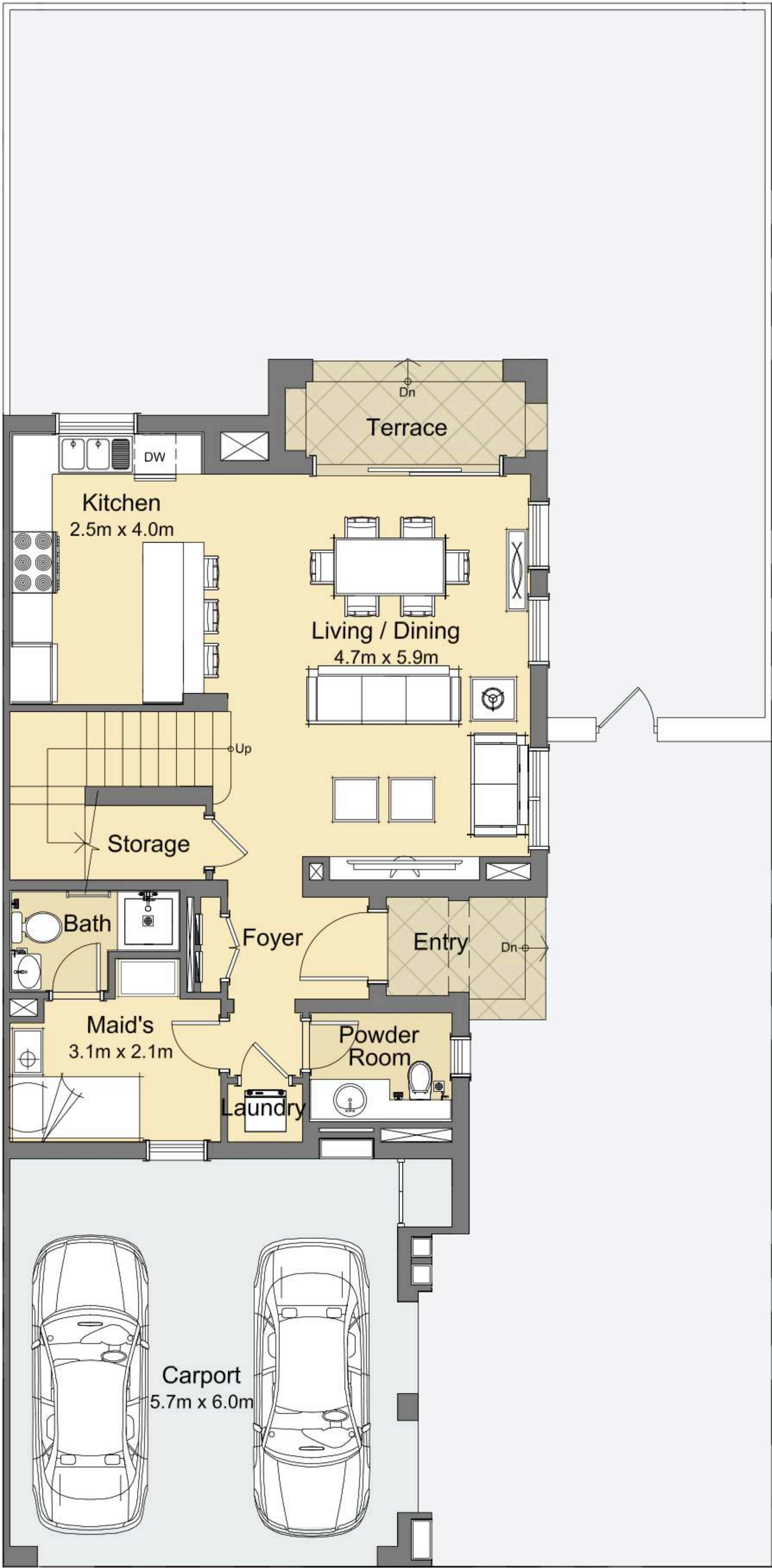
GROUND FLOOR
