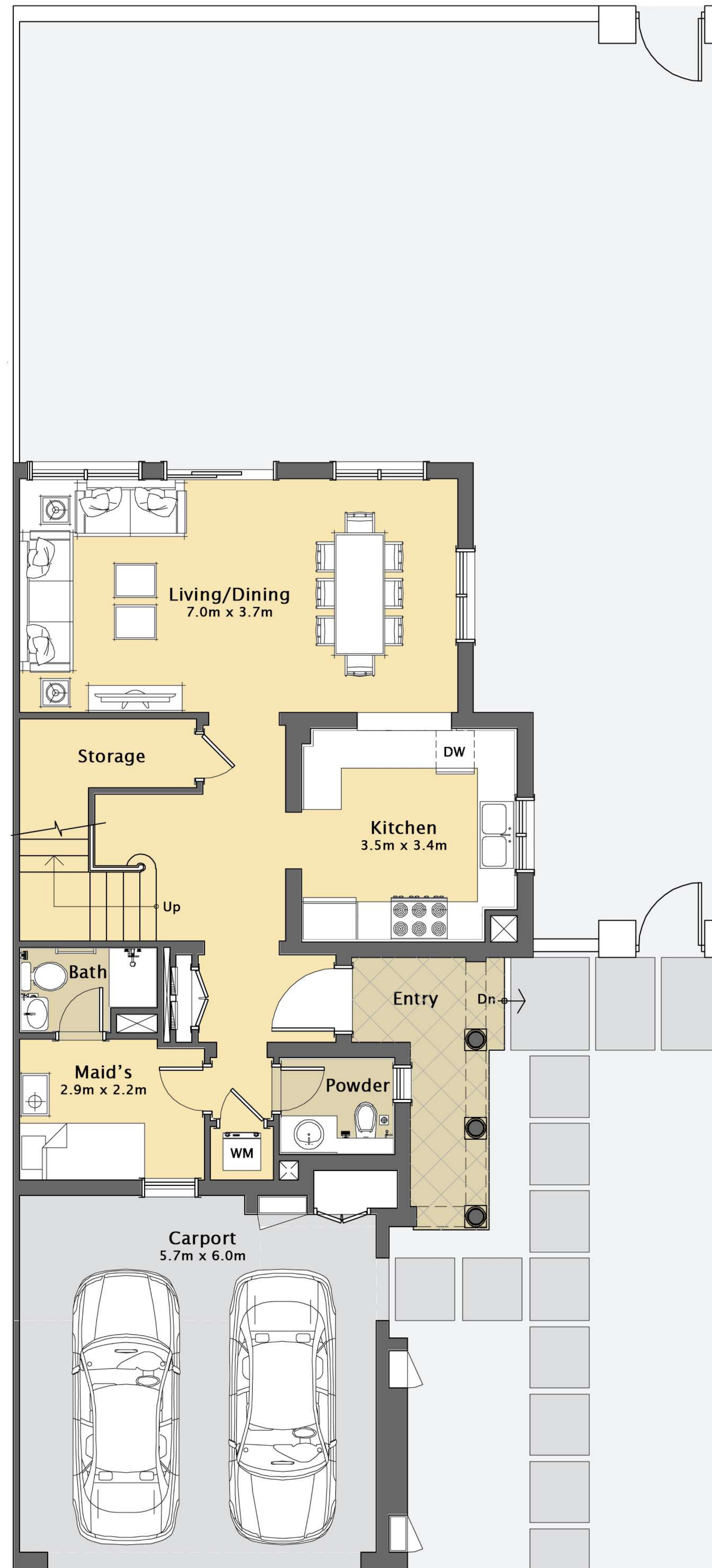
GROUND FLOOR
