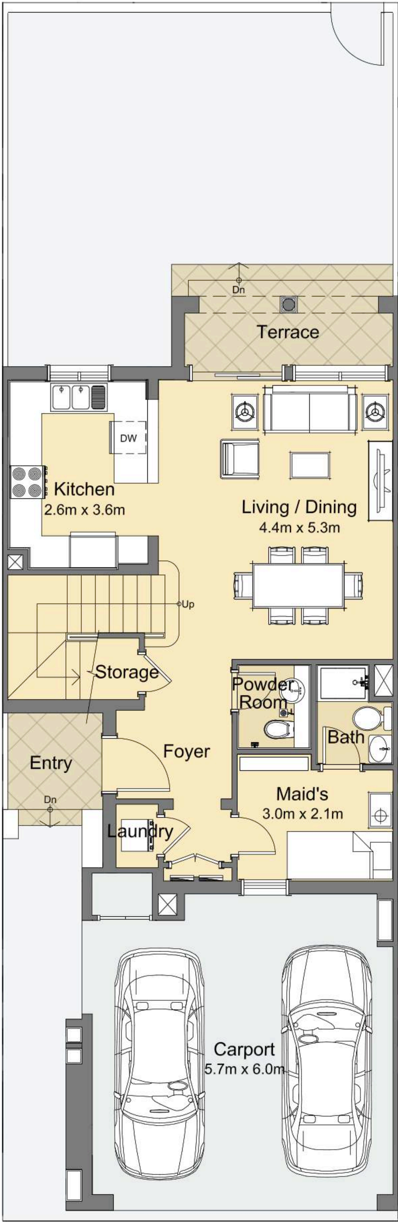
GROUND FLOOR
