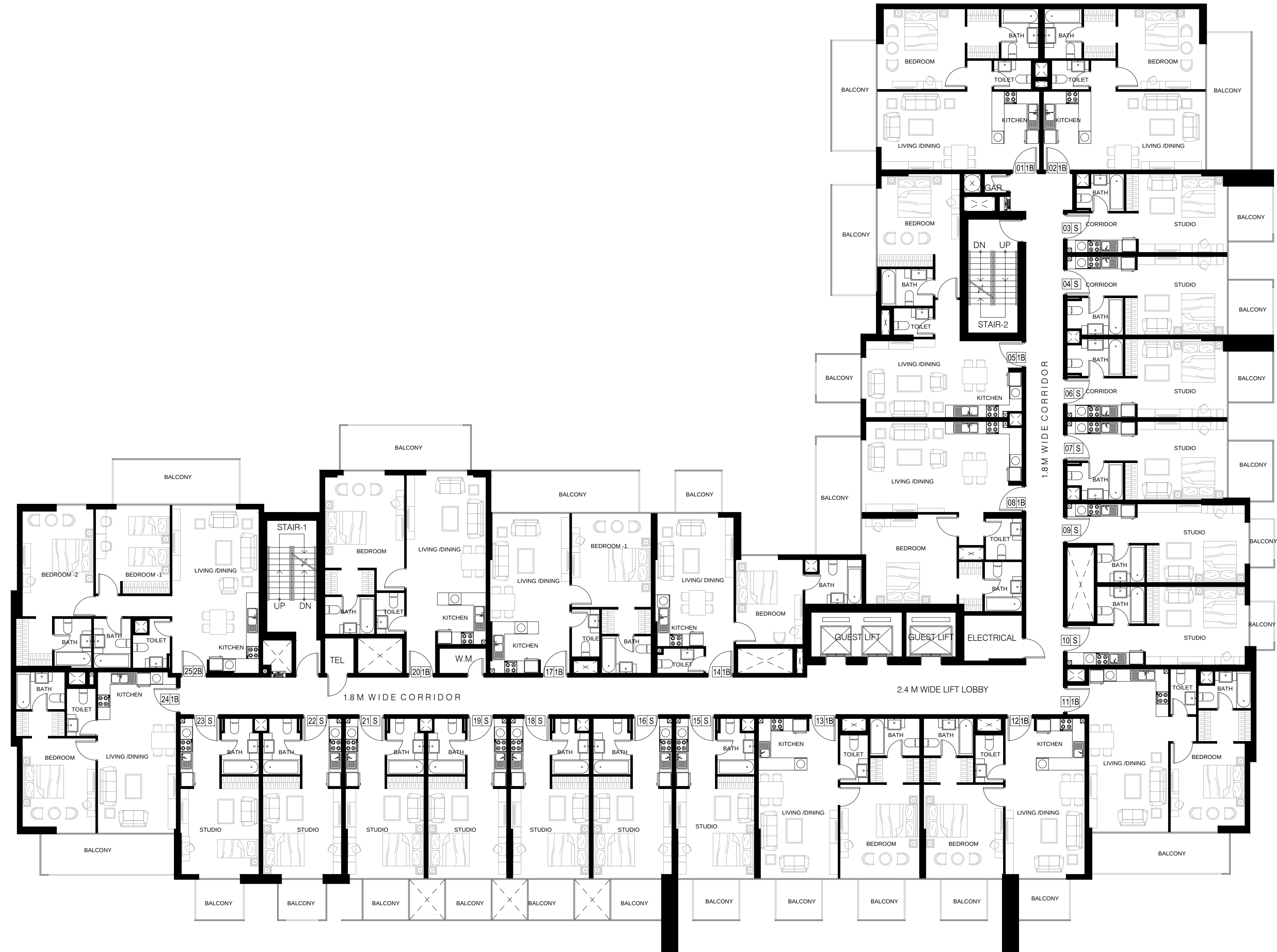
TYPICAL FLOOR
