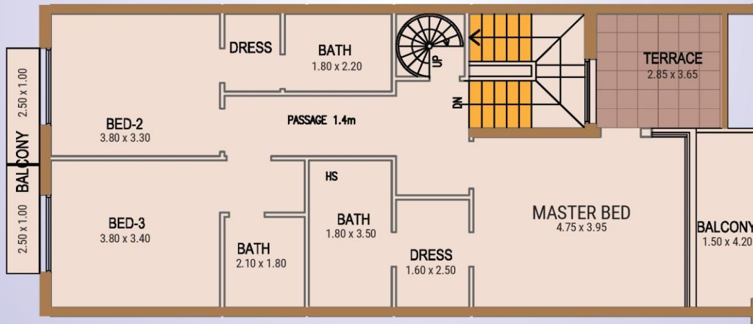
First Floor
